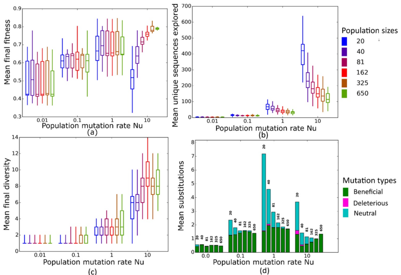
Figure 4. Simulated evolution of sequences with secondary structure I (StrI, Table 1) at varying population mutation rates N\mu and population sizes. We randomly-selected a low-fitness sequence to initialize each simulation, and then simulated 800 generations of mutation and selection. We performed 50 replicate simulations for each mutation rate (horizontal axes) and population size (see Methods). Boxplots show (a) final mean population fitness, (b) total unique sequences explored, and (c) final population diversity (number of unique sequences at generation 800). Each box encloses the second and third quartiles of the 50 replicates, the center line corresponds to the median, and the whiskers depict the minimum and maximum values obtained from any replicate, excluding the outliers. (d) Mean numbers of unique beneficial, deleterious, and neutral substitutions (green, pink, and cyan) are summarized as bars for the 50 replicates at each mutation rate (horizontal axis) and population size (labels above bars).
