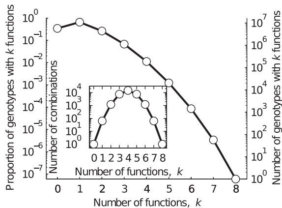
Figure 2. Multifunctional regulatory circuits. Each data point depicts the proportion and number of genotypes with k functions. The data include all k -functions. The line is provided as a visual guide. Note that there are more circuits with k=1 function than with k=0 functions, implying that a randomly selected circuit is more likely to be viable than not. Also note that any circuit with k functions will be included in the count of the number of circuits with between 1 and k-1 functions. The inset shows the number of observed combinations of functions (open circles) and the total number of possible combinations (solid line) of k functions. Note the logarithmic scale of all y-axes.
