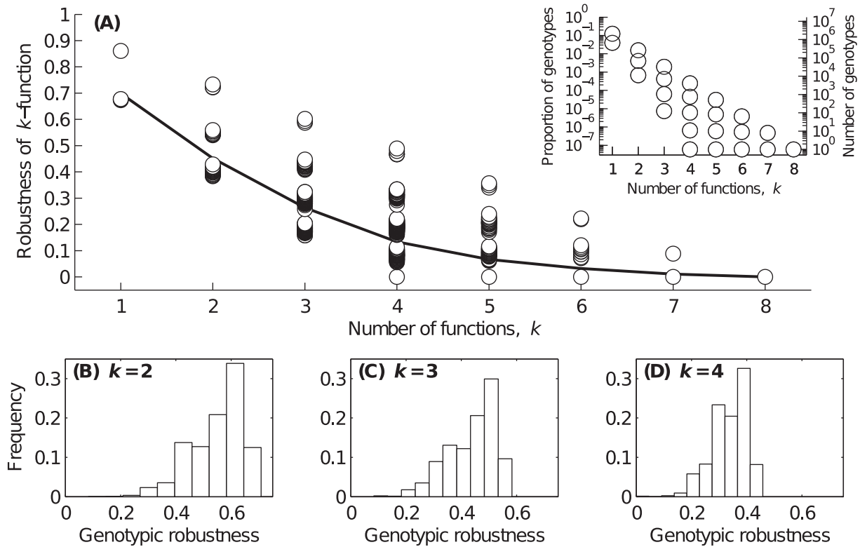
Figure 3. Robustness and multifunctionality. (A) The robustness of a k -function is shown in relation to the number of functions k . Each data point corresponds to the genotype set of a specific combination of k functions. The data include all k -functions. The solid line depicts the average robustness of a k -function. The inset shows the proportion and number of genotypes in the genotype set of a k -function, as a function of k . Note the logarithmic scale of the y-axes. (B–D) Distributions of genotypic robustness for (B) k=2 , (C) k=3 , and (D) k=4 . For each k , we show data for a single genotype network.
