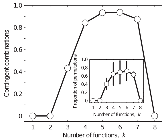
Figure 5. Historical contingency in multifunctional regulatory circuits. Each data point shows the proportion of combinations of k functions that exhibit contingency, as a function of k . The line is provided as a visual guide. The inset shows the average proportion of the k! permutations of each combination of k functions that exhibit contingency. Error bars denote one standard deviation. doi:10.1371/journal.pcbi.1003071.g005
