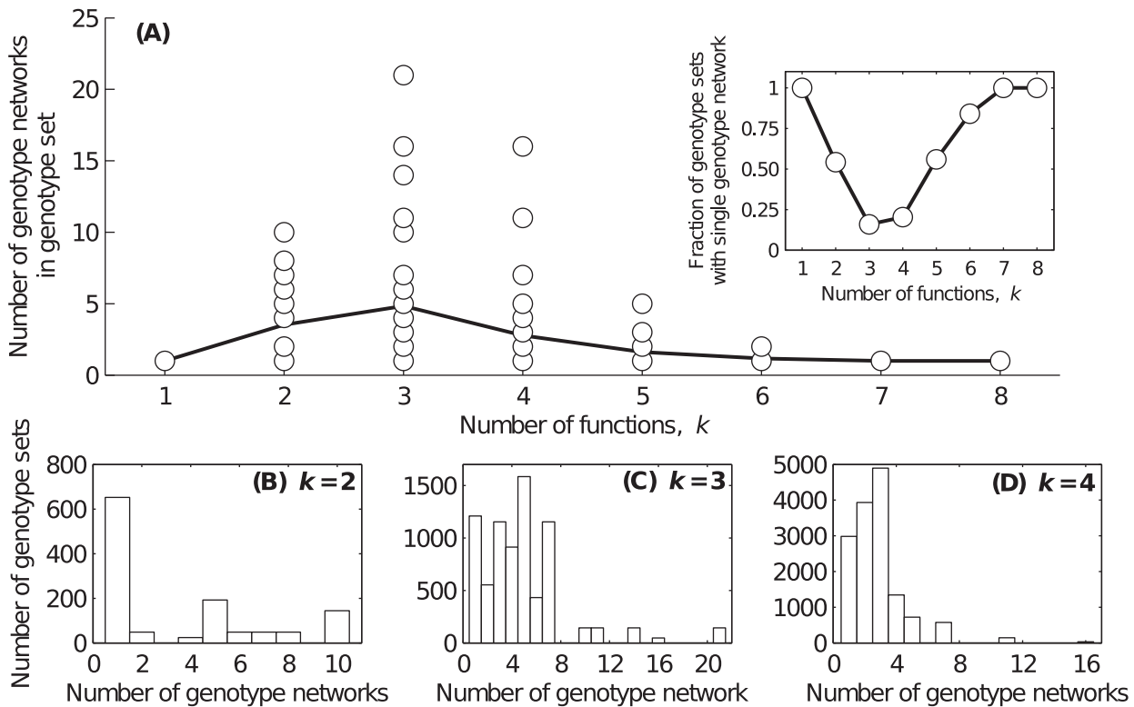
Figure 4. Genotype set fragmentation. (A) Each data point shows the number of genotype networks in the genotype set of a specific k -function. The data include all k -functions. The solid line depicts the average number of genotype networks per k -function. The inset shows the proportion of genotype sets that comprise a single genotype network, as a function of k . (B–D) The distributions of the number of genotype networks per genotype set for (B) k=2 , (C) k=3 , and (D) k=4 . doi:10.1371/journal.pcbi.1003071.g004
