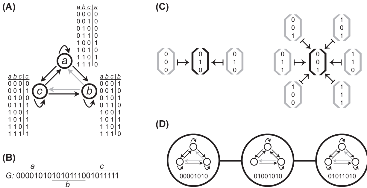
Figure 1. Schematic illustration of the Boolean model of gene regulatory circuits. (A) A Boolean circuit with N = 3 genes ( a, b, c ), which are represented as open circles. Two genes are connected by a directed edge a \rightarrow b if the expression of gene b is regulated by the product of gene a . Gene expression is binary, such that genes are either expressed (1) or not (0). The signal-integration logic of each gene is shown as a lookup table that explicitly maps all 2^N possible input expression states to an output expression state, implicitly determining the circuit's topology. In the hypothetical circuit shown, the expression state of gene a is independent of the expression state of gene b , so b \rightarrow a is a non-existing regulatory interaction (gray arrow), whereas c \rightarrow a and a \rightarrow a are both existing regulatory interactions (black arrows). (B) The wiring diagram and signal-integration logic of the entire circuit can be represented by a single vector G that is constructed by concatenating the rightmost columns of the lookup tables of the individual genes in panel (A). The vector G corresponds to the circuit's genotype. (C) The circuit in (A) maps all of the 2^3 = 8 possible initial states S_0 (gray brackets) onto two distinct stable equilibrium expression states S_\infty (black brackets). This circuit therefore can have up to k = 2 functions, and can express such a "bifunction" in 6 \times 2 = 12 different ways, since 6 initial states map to one equilibrium expression state and the other 2 initial states map to another equilibrium expression state. (D) In a genotype network, vertices represent circuits and two vertices share an edge if the genotypes G differ by a single element, yet have the same functions. Here, the genotype network corresponds to circuits with the bifunction F^{(1)} : (\langle 0, 0, 0 \rangle \mapsto \langle 0, 1, 0 \rangle) , F^{(2)} : (\langle 0, 1, 1 \rangle \mapsto \langle 0, 0, 1 \rangle) . For visual clarity, each circle only shows the first 8 binary digits of G , which represent the signal-integration logic of gene a . Note how changes in G may implicitly translate to changes in circuit topology. doi:10.1371/journal.pcbi.1003071.g001
