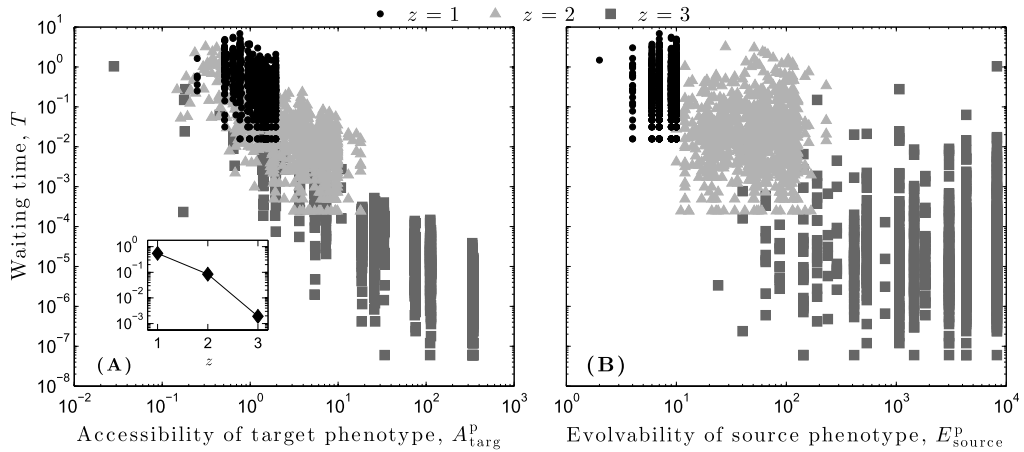
Figure 7. Waiting time of a random walk T = S/2^L as a function of (A) the target phenotype's accessibility A^P_{\text{targ}} and (B) the source phenotype's evolvability E^P_{\text{source}} , for each of the three dynamical regimes: ordered ( z = 1 ), critical ( z = 2 ), and chaotic ( z = 3 ). The inset in (A) depicts the average waiting time T as a function of z . Lines are provided as a guide for the eye.
