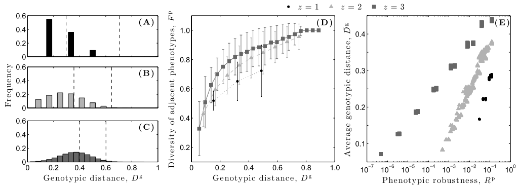
Figure 5. Distribution of the genotypic distance D^g between randomly sampled pairs of genotypes from focal genotype networks in each of the three dynamical regimes: (A) ordered ( z = 1 ), (B) critical ( z = 2 ), and (C) chaotic ( z = 3 ). The dashed vertical lines represent one standard deviation from the mean of the corresponding null distribution (see text). (D) Diversity of adjacent phenotypes F^p as a function of genotypic distance D^g . Data are offset in the horizontal dimension for visual clarity. Error bars denote one standard deviation from the mean. (E) Average genotypic distance \bar{D}^g per genotype network, as a function of phenotypic robustness R^p .
