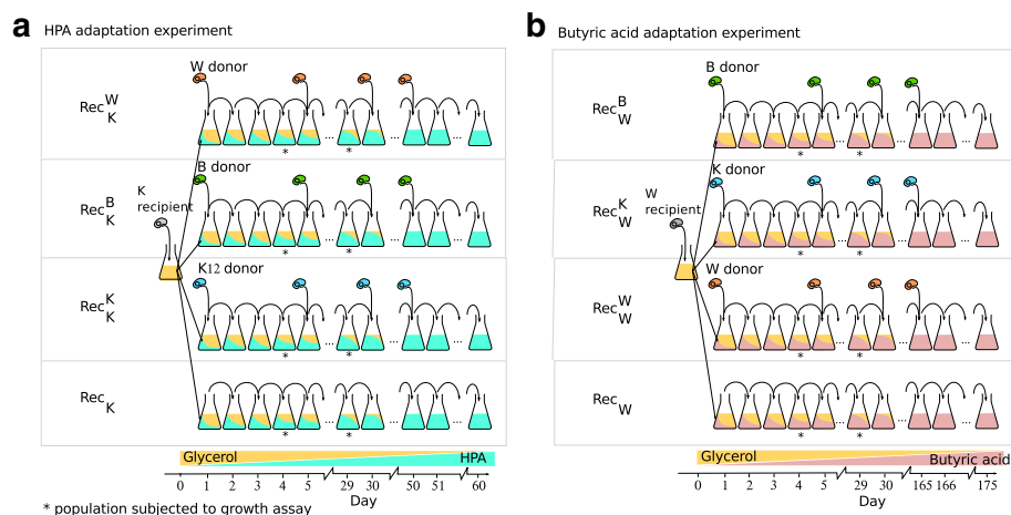
Fig. 1 Experimental design of both evolution experiments. a We evolved multiple replicate populations of the K recipient strain on HPA for 60 serial transfer cycles (< 400 generations). Specifically, we established populations that we periodically exposed to W donor cells (6 replicate populations, \text{Rec}_K^W ), to B donor cells (6 replicates, \text{Rec}_K^B ), to K donor cells (6 replicates, \text{Rec}_K^K ), and to no donor cells (6 replicates, \text{Rec}_K ; see Methods). b We evolved multiple replicate populations of the W recipient strain on butyric acid for 175 days (~ 1155 generations). Specifically, we established populations that we periodically exposed to B donor cells (6 replicate populations, \text{Rec}_W^B ), to K donor cells (6 replicates, \text{Rec}_W^K ), to W donor cells (6 replicates, \text{Rec}_W^W ), and to no donor cells (6 replicates, \text{Rec}_W ). For both experiments, we seeded the recipient populations from a single overnight culture of the ancestral recipient (gray cell cartoon at the left of each panel) grown in glycerol. Everyday, we transferred each evolving population to fresh growth medium (Additional file 35: Table S4) by 100-fold dilution (black arrows). Every five days, we prepared glycerol stocks, screened for contaminations, monitored adaptation via growth assays, and added the appropriate donor to the evolving population (Methods). Over the course of the experiment, we gradually replaced glycerol (dark yellow) with HPA (cyan) ( a ) or butyric acid (pink) ( b ) in the growth medium, until only the novel carbon source was present. Then, we evolved the populations for 10 more days in the novel carbon source to ensure that the populations could grow exclusively on the novel carbon source
