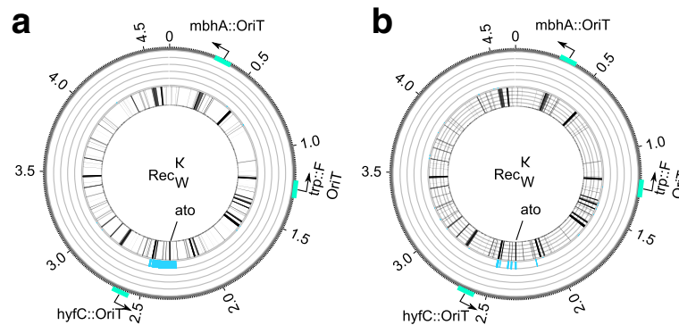
Fig. 5 Circos plots of the distributions of horizontally transferred genes among butyric acid-evolved clones. a Putatively horizontally transferred genes among W recipients exposed to K donors in Rec_W experiments during adaptive evolution on butyric acid. The circos plots show several concentric circles. The outermost circle (dark grey line) indicates genomic coordinates (in Mb) from the origin of replication (marked as 0), the location of the oriT located in the F-plasmid integrate, and the other two oriT sequences (green rectangles). The innermost circle shows a radial black bar at each genomic location where a gene is present in the ancestral donor (K) but not the ancestral recipient (W) genome (in K genome coordinates). The middle circle shows the number of populations that have acquired one or more genes in at least one of the sequenced clones of the population at that location in the K donor, as the height of each green radial bar (maximum height corresponding to five populations). b Analogous to (a) , except that the middle circle now reports the number of sequenced clones that have acquired the gene at that location only for genes that occur both in the ancestral W recipient and the ancestral K donor. Note that all gene locations are in coordinates of the E. coli K12 reference genome. All data are based on sequence coverage based estimation of horizontally transferred genes (Methods). The location of the ato operon (at 2.32 Mb), which is involved in butyric acid degradation is marked at the innermost circle
