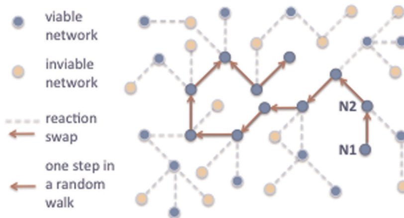
Figure 5. Exploration of a metabolic network space. Metabolic networks can be viewed as subsets of enzyme-catalyzed metabolic reactions in a global reaction set. Formally, they can be represented as binary vectors listing the reactions catalyzed by enzymes in an organism, as indicated for two hypothetical metabolic networks (N1, N2) in the figure. Metabolic phenotypes are computed from metabolic networks using FBA. They can be represented as binary vectors indicating the carbon sources (i.e.: alanine, glucose, melibiose,...) on which a network is viable, that is, on which it can synthesize a given set of (biomass) molecules. Neighboring networks (blue circles linked by edges) differ by a single reaction swap (edges between circles) that leaves the metabolic phenotype unchanged. A reaction swap consists of two changes: one random reaction addition (R4 in the example) and one random reaction deletion (R3 in the example). A series of successful reaction swaps is called a random walk (indicated by red arrows). The Markov Chain Monte Carlo (MCMC) technique allows one to randomly sample networks with a given phenotype by generating long random walks through genotype space, where each step in a walk consists of a reaction swap. The advantage of using reaction swaps is that they leave the number of reactions constant.
