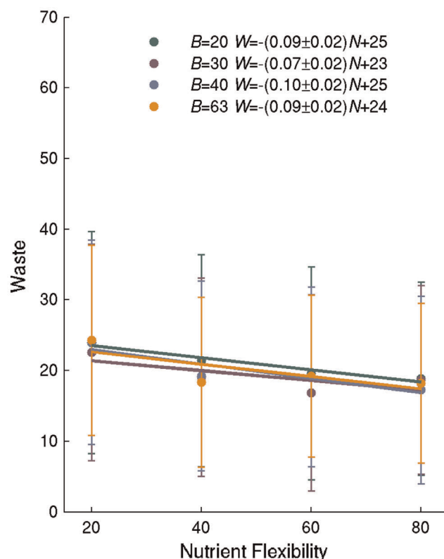
Figure 3. Waste production decreases with nutrient flexibility.
