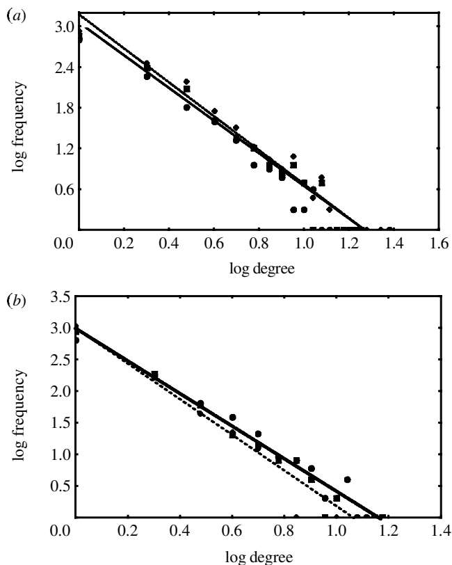
Figure 3. Duplication and divergence, taken together, do not affect degree distribution. (a,b) A double logarithmic plot of the degree distribution in the protein network (circles) as reported by Uetz et al. (2000), and in the same network after 1000 (squares) and 2000 (diamonds) gene duplications. With an effective rate of 8.3 \times 10^{-4} \text{ gene}^{-1} \text{ Myr}^{-1} , ca. 1000 gene duplications are expected in the network every 1.2 Gyr. The results stem from a numerical simulation of network evolution, where I repeatedly duplicated individual genes chosen at random from the network, and let interactions diverge as follows after each duplication. (a) Asymmetric divergence. Functional divergence between gene duplicates generally occurs asymmetrically, i.e. one gene product retains more molecular interactions than the other. This is the divergence pattern observed empirically (Wagner 2002). To emulate this scenario, I chose one of the two duplicate genes at random, and eliminated each interaction of this gene independently with probability 1 - f = 0.85 . This procedure ensures not only that divergence is asymmetric, but also that an average of 15% of shared interactions remain after the duplication, a value close to the maximum of that observed in the empirical data (see text). The exponents \gamma of the degree distribution, P(d) \propto d^{-\gamma} are as follows. Circles, protein interaction network ( \gamma = 2.55 ); squares, after 1000 duplications (1200 Myr; \gamma = 2.25 ); diamonds, after 2000 duplications (2400 Myr; \gamma = 2.29 ). The 95% CIs of these exponents are greater than 0.35 in all three cases shown. Thus, the distributions are statistically distinguishable. (b) Symmetric divergence. I chose and eliminated one of the two interactions in each redundant interaction pair of two gene duplicates (figure 2b) with probability of one-half. After this procedure, the expected number of retained interactions per gene is half the number before duplication. In this sense, divergence is symmetric. I eliminated proteins without remaining interactions after this procedure. Circles, protein interaction network ( \gamma = 2.55 ); squares, after 1000 duplications (1200 Myr; \gamma = 2.58 ); diamonds, after 2000 duplications (2400 Myr; \gamma = 2.82 ).
